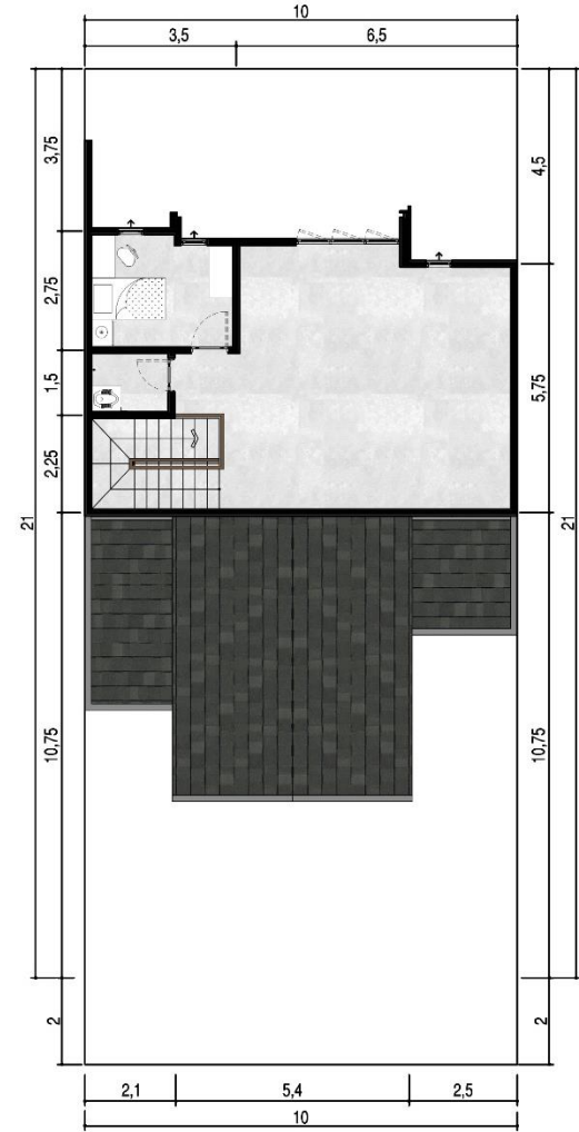
THIRD FLOOR SCALE 1 : 100
