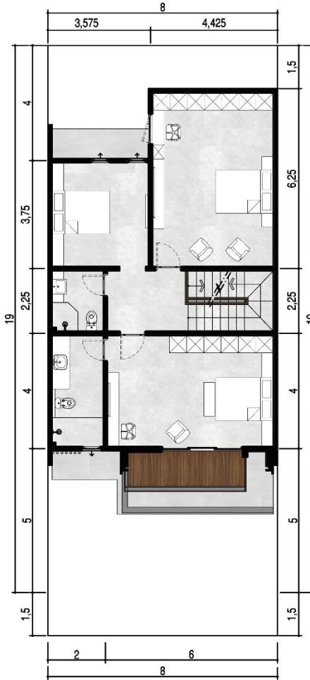
SECOND FLOOR SCALE 1:100
