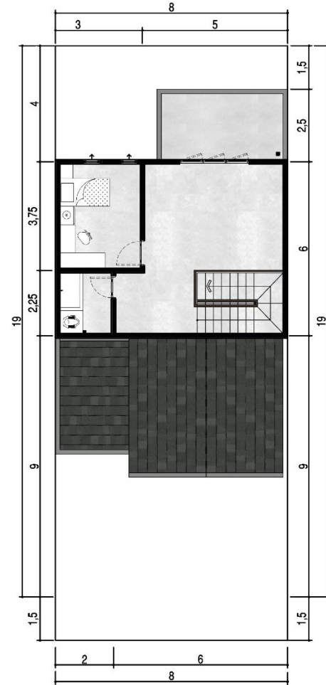
THIRD FLOOR SCALE 1:100
